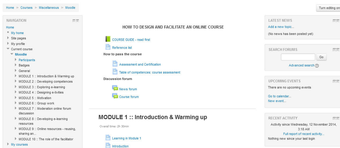
Figure 3-8 Course Page
