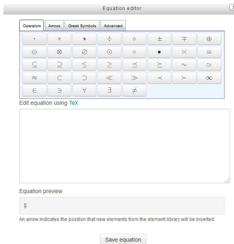
Figure 6-3 Equation Editor
